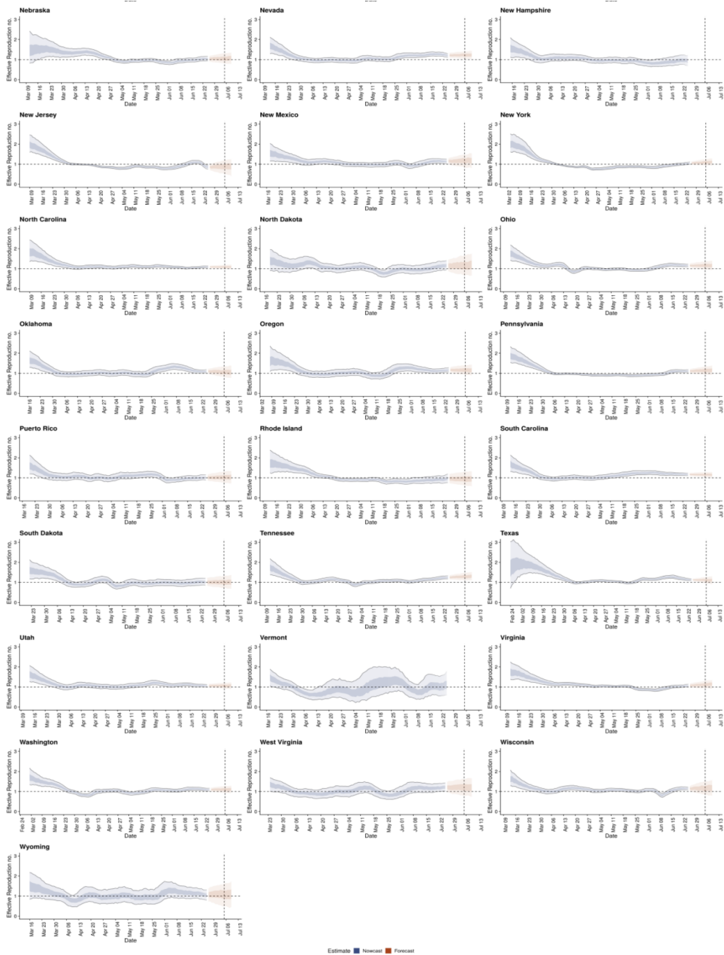
Figure 2: Estimated \mathcal{R}_t for US States (COVID-19) from epiforecasts.io - part II
