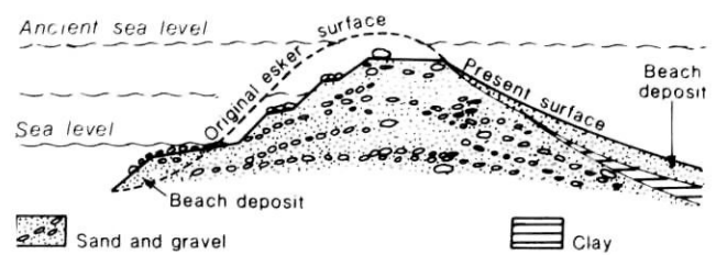
FIGURE 1. Simplified scheme of cross-section of an esker running parallel to the beach in Southern Finland, a region with rapid land uplift.
