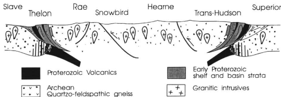
Figure 6 Schematic cross-section of the assembly of Archean terrains in the Proterozoic.
