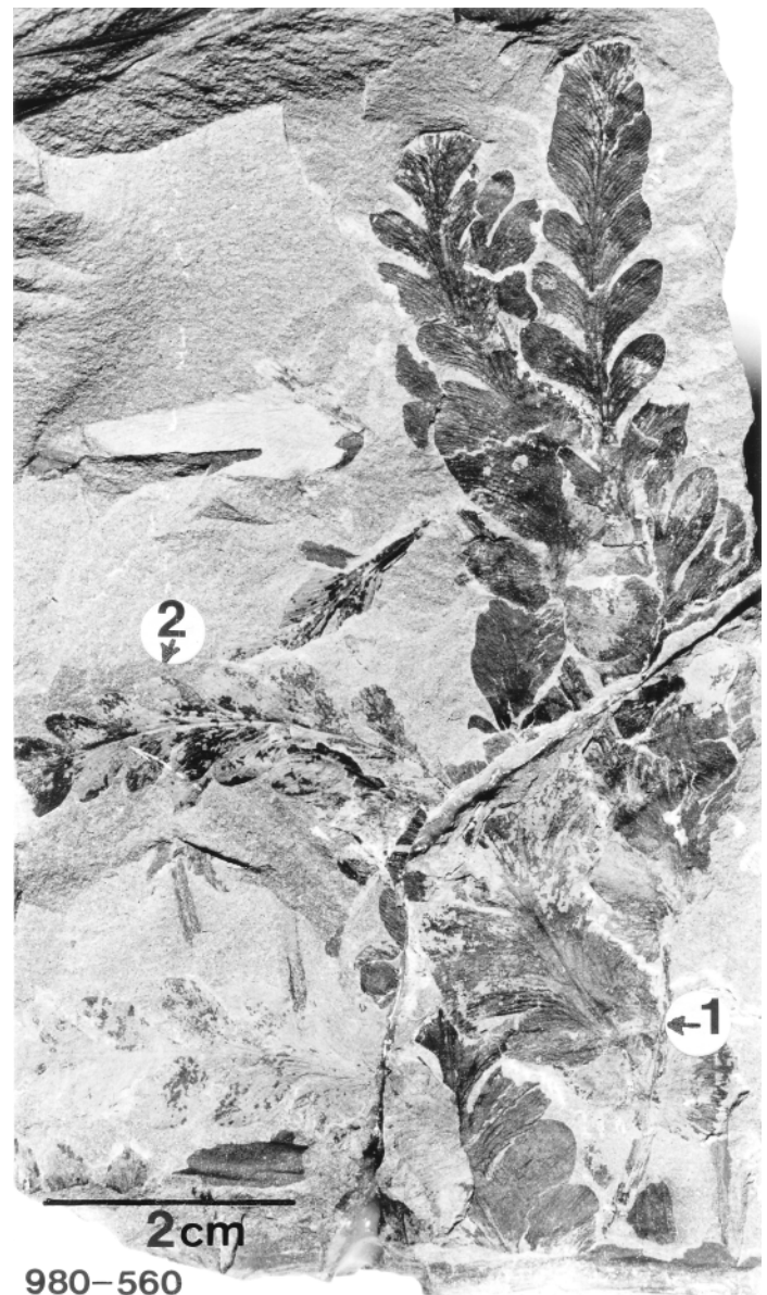
Fig 8 " Odontopteris subcuneata ", M. scheuchzeri . Basal part (arrowed "1") is typical M. scheuchzeri with epicuticular hair, whereas the laciniate apex arrowed "2") is typical " O. subcuneata " without hair. 980-560; Lloyd Cove Seam.
