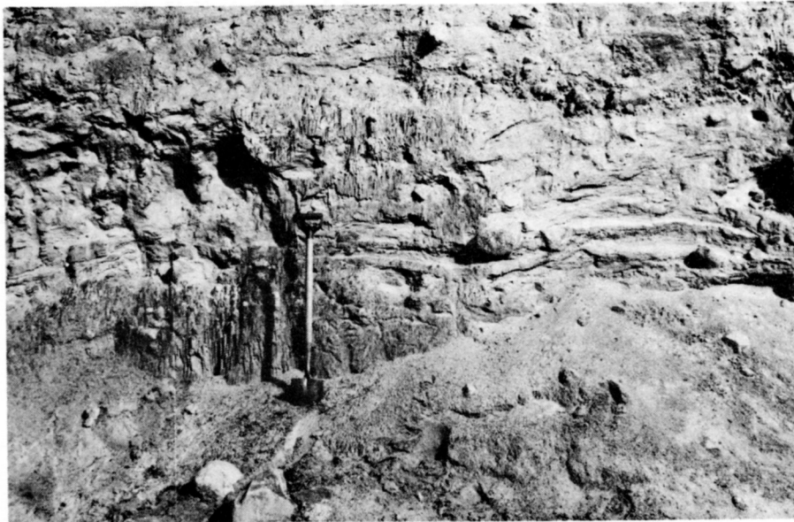
Plate 3. Granite Till C exposed 3 km north of Chester. The horizontal gravel/sand beds indicate re-working by glacial meltwater during till deposition.
