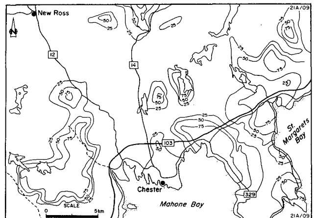
Fig. 9b. Clast lithology map showing the contoured percentages of Sandy Lake Monzogranite clasts in Granite Till B and Granite Till C.
