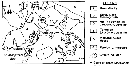
Fig. 3. Location of till sections A and B in relation to bedrock of the South Mountain Batholith.
