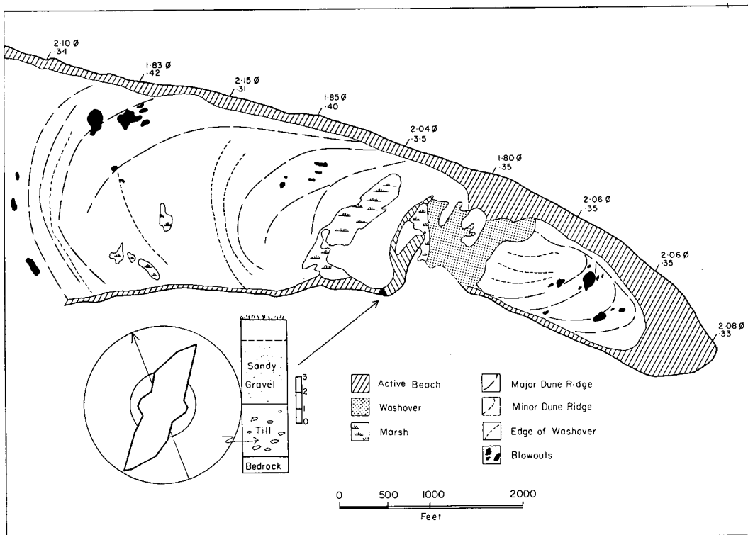
Figure 3 - Occurrences and textural details of dunes southeast of large washover fan; Hog Island (see Fig. 1 for location).
