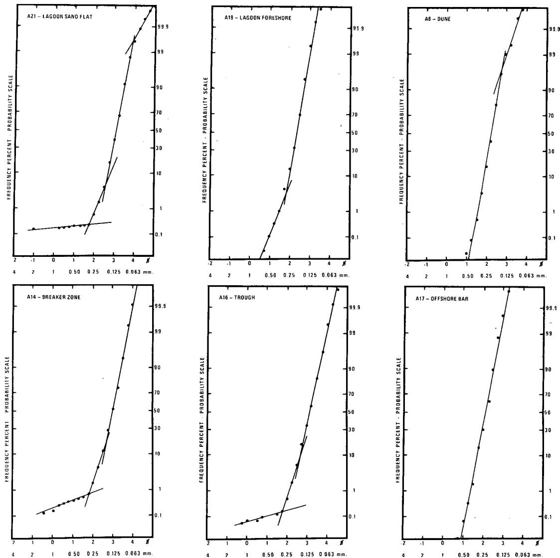
Figure 9 - Size frequency characteristics of selected samples plotted on arithmetic probability paper. Log normal components of each sample have been drawn in by eye. The locations of the three beach samples (A14, A16, A17) are shown in Fig. 4.
