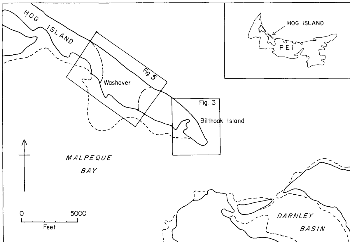
Figure 1 - Location map of Hog Island, with rectangles showing area of Figs. 3 & 5.
