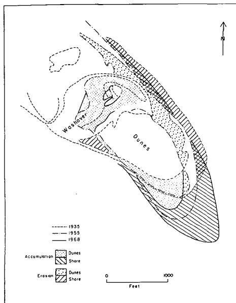
Figure 5 - Extension of shoreline of Hog Island for 600 in southeast direction.
