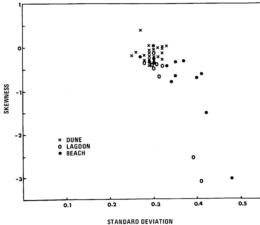
Figure 7 - Bivariate plot of sorting (standard deviation) vs. skewness for the lagoon, beach and dune samples.
