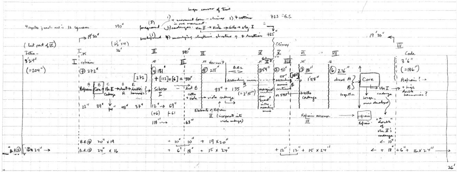
Figure 14. Cherney's overview diagram for the form of the quartet, excerpt from sketch
