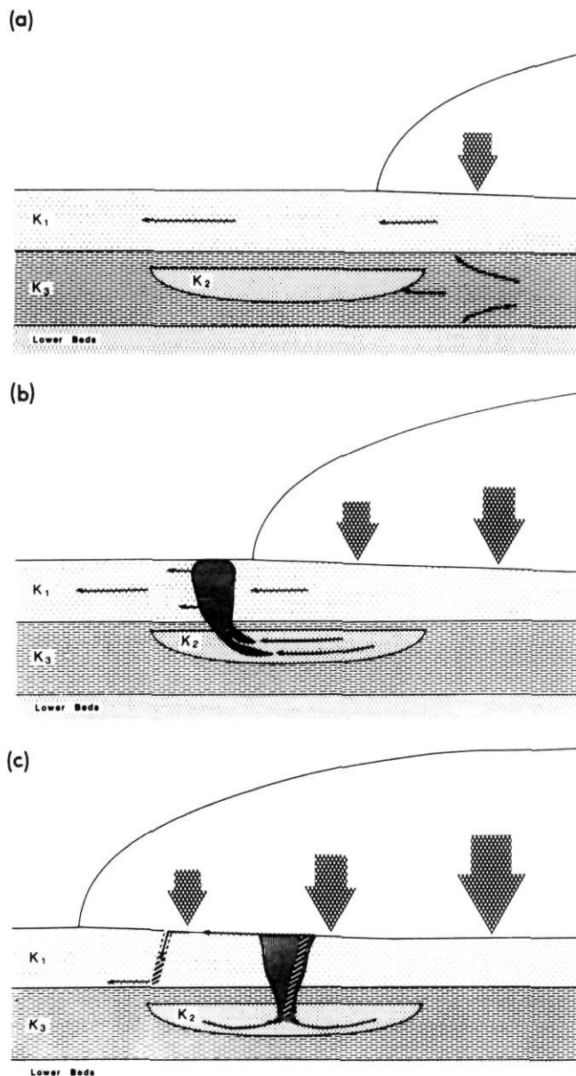
FIGURE 14. Model illustrating the increase in porewater pressure due to increase in load from advancing ice. As load is increased porewater is expelled from units with high conductivity (K 1 ) but may be trapped in confined aquifers (K 2 ) within less permeable units (K 3 ). At some critical load, pore pressure may be sufficient to cause expulsion through a thin confining unit as in (b) or the confined aquifer may experience fracturing (c) resulting in catastrophic release and fluidization along the fracture system. Fluid may be free to exit the glacier margin or be injected into other fracture systems, depending upon hydraulic gradient and subglacial thermal conditions.
