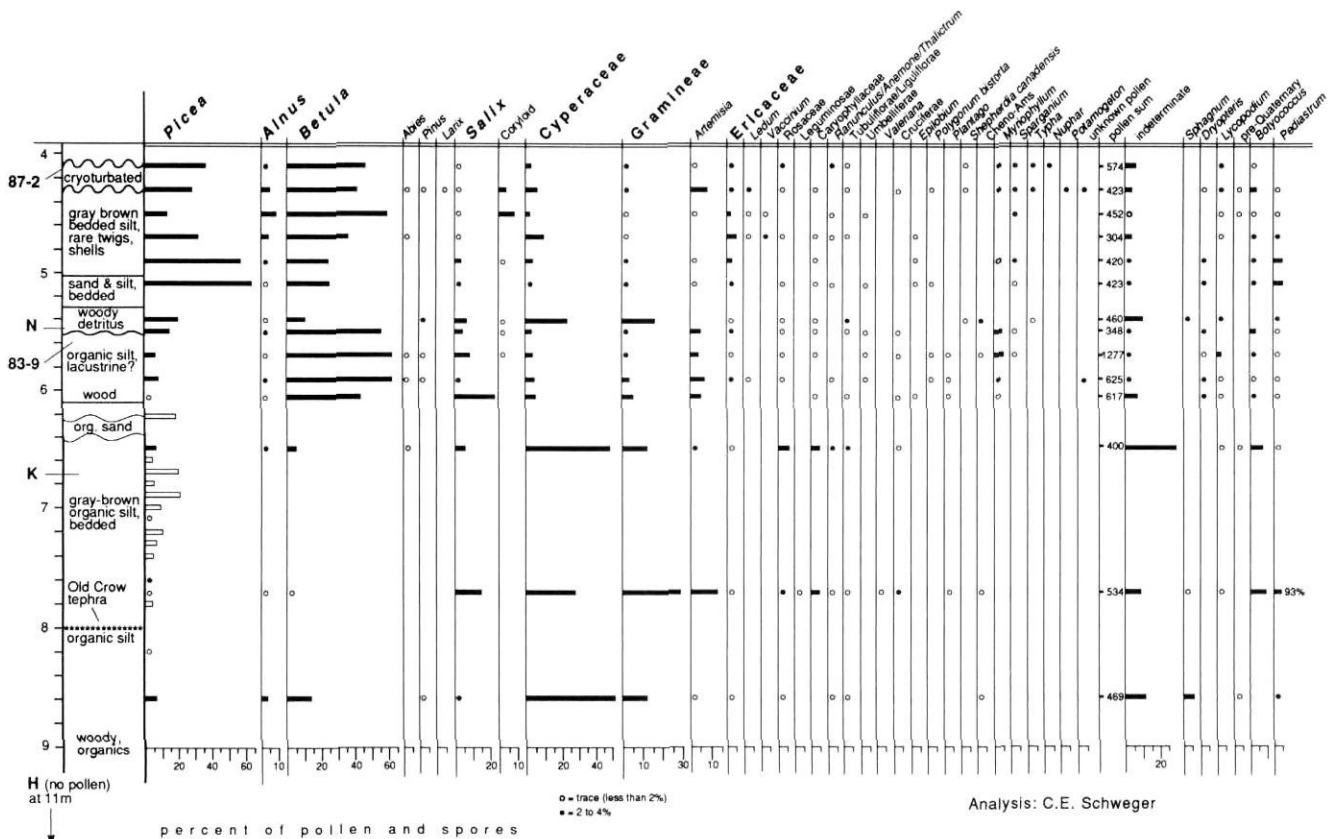
FIGURE 5. Pollen diagram from part of Unit 4 at Station 4 (Fig. 2). Depth is shown in metres below base of Unit 5 and follows numbers shown in Figure 4.
