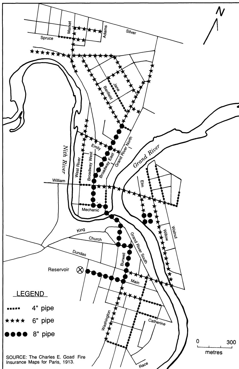
Figure 4: The Paris Water-works System, 1913
