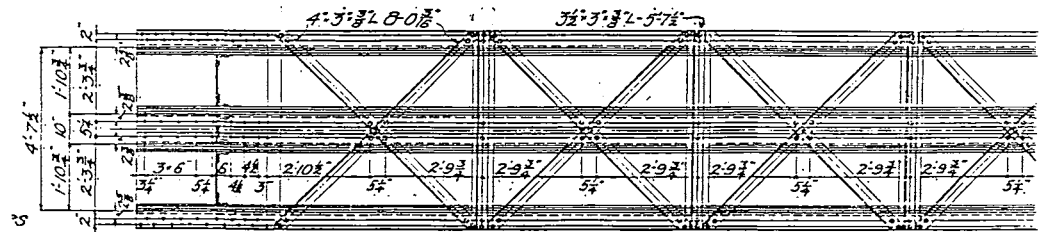
PLAN ON A-A
