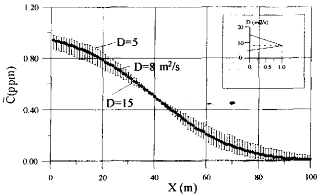
Figure 2 Distribution du \hat{C} flou en dispersion convective unidimensionnelle. Distribution of fuzzy \hat{C} for one-dimensional convective dispersion.
