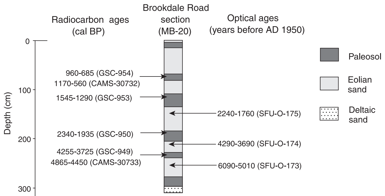
FIGURE 3. Chronostratigraphic profile of the Brookdale Road section (MB-20) showing calibrated radiocarbon ages of David (1971) and Wolfe et al. (2000), and optical ages from this study. Uncertainties in the ages are shown at \pm 2\sigma .
