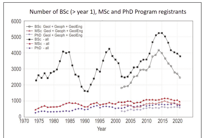
Figure 5. The number of geoscience students in Canadian universities from 1974 to 2021 (courtesy of the Council of Chairs of Canadian Earth Science Departments; cccesd.acadiau.ca/ ). The solid symbols include all students in their respective programs (BSc, MSc and PhD), the hollow symbols include the students in geology + geophysics + geological engineering fields minus the environmental sciences students. This separation was started in 2002. Note that there has been a drop of 1700 (42%) in 2021 from 4200 undergraduate geoscience students in 2014.
