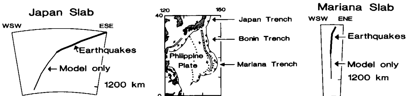
Figure 4 The Mariana and the Bonin Trenches are the eastern boundaries to the Philippine Plate. The centre panel shows the major tectonic elements: underthrusting and trench axes - solid lines with barbs; spreading axes - double lines and arrows; ridges - dots. (This has been re-drawn, greatly simplified, from Karig and Rankin, 1983, fig. 1). The left and right panels show the difference between the down-going slabs of the Japan and Mariana convergences — the Mariana slab dips nearly vertically. Note that there is no vertical exaggeration. The upper part of the down-going slabs, shown in heavy line, are well-defined by earthquakes; the lower part of the slabs, shown as lighter line, are interpretations from travel-time residuals (Creager and Jordan, 1986). Note the discussion concerning this - it bears on mantle convection (Frohlich, 1989). (These panels have been re-drawn, greatly simplified, from Creager and Jordan, 1986, fig. 5).
