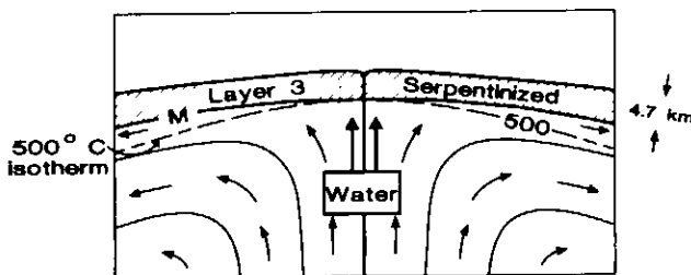
Ocean crust as serpentinized mantle Hess's ideas of 1962
