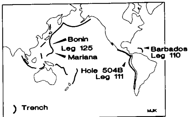
Figure 1 Location diagram. Leg 110 of the Ocean Drilling Program occupied sites on the Barbados Ridge complex and adjacent ocean floor in the region of the convergent boundary between the Atlantic Plate and the Caribbean Plate. Leg 125 occupied sites on the convergent boundary between the Pacific Plate and the Philippine Plate. The figure also shows the sites of most of the world's oceanic trenches.
