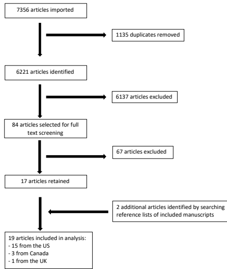
Figure 1. PRISMA diagram
