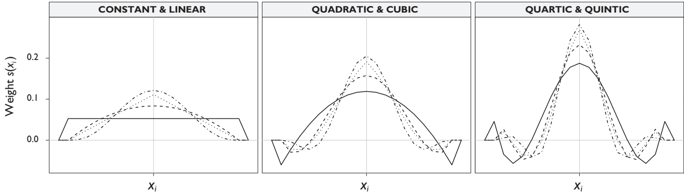
FIGURE 2 SMOOTH WEIGHTS s(x_i) , FOR OBSERVATION i IN THE CENTRAL REGION, COMPUTED WITH \lambda = 19 FOR RECTANGULAR (SOLID LINE), TRIANGULAR (DOTTED LINE), EPANECHNIKOV (DASHED LINE) AND TRIWEIGHT (DOTDASHED LINE) WEIGHT FUNCTIONS
