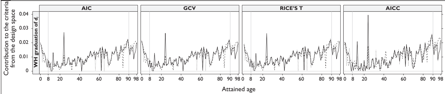
FIGURE 11 POINTWISE CONTRIBUTION TO THE CLASSICAL CRITERIA FOR THE WHITTAKER-HENDERSON MODEL TARGETING THE NUMBER OF DEATH, D , DUTCH FEMALE POPULATION, 2008. QUADRATIC FIT (DASHED LINE), CUBIC FIT (FULL LINE) AND QUARTIC FIT (DOTTED LINE)
