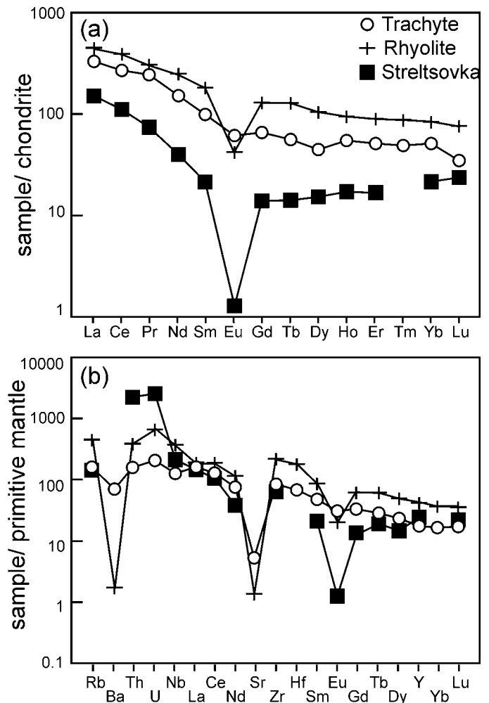
Fig. 7. (a) Chondrite-normalized REE patterns of the averages of trachyte ( n = 7 ) and rhyolite ( n = 8 ) samples from the Cumberland Hill Formation and rhyolite from Streltsovka ( n = 1 ; Chabiron et al. 2003); (b) Primitive mantle-normalized multi-element plots of the average of trachyte ( n = 7 ) and rhyolite ( n = 8 ) samples from the Cumberland Hill Formation and rhyolite from Streltsovka ( n = 1 ; Chabiron et al. 2003). Normalizing values are after Sun and McDonough (1989).
