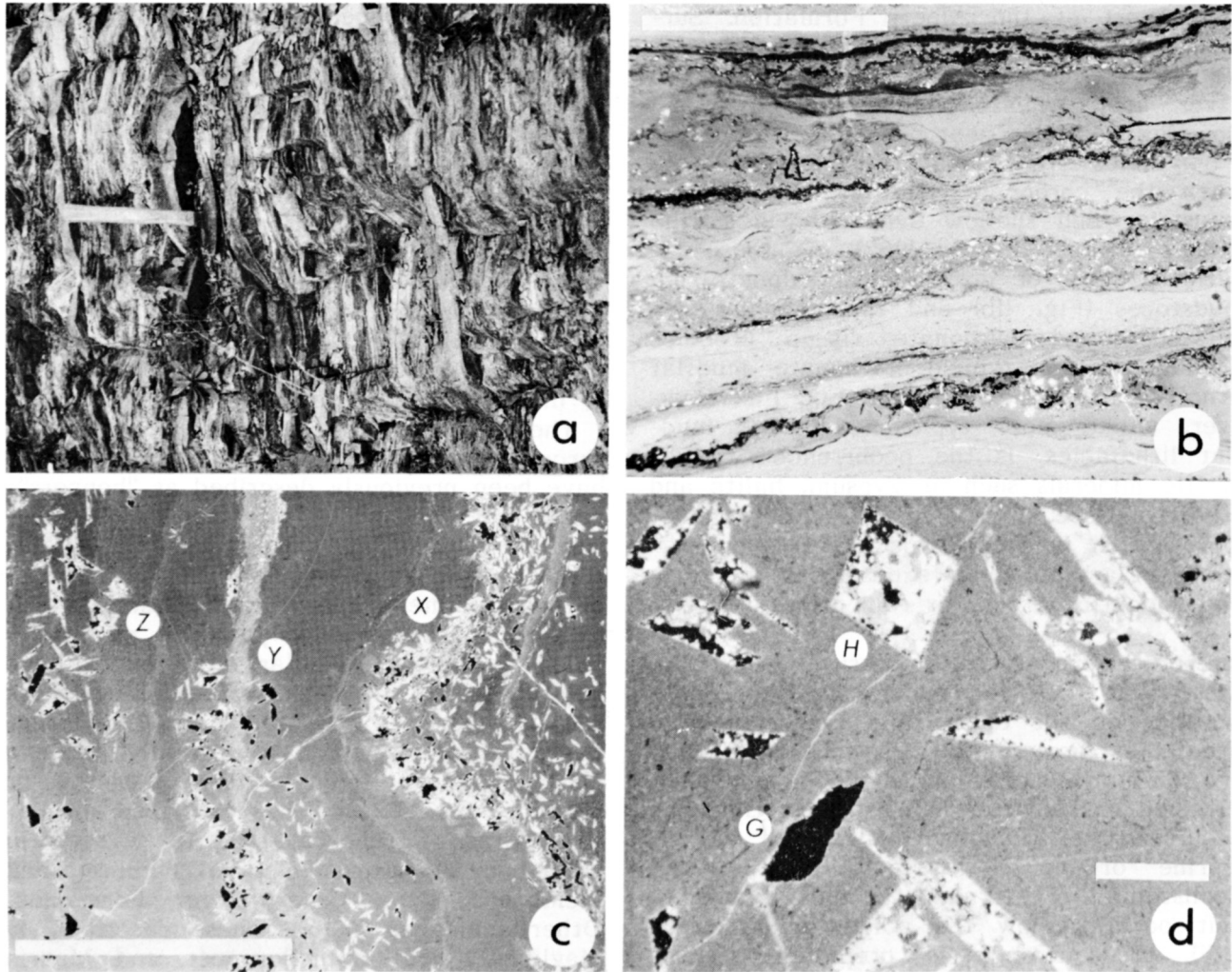
Fig. 10 - Shallow evaporitic lacustrine lithofacies, Albert Formation, Mocton Subbasin. a) Thinly interbedded shale, silty shale and mudstone with lighter coloured storm sheet sandstones. Stratigraphic top to left and hammer for scale. b) Photomicrograph of massive to parallel laminated sulphate-rich mudstone with abundant disseminated evaporite crystal molds. c) Photomicrograph of massive evaporitic mudstone with continuous crusts (X), discontinuous crusts (Y) and intrasediment crystal molds (Z) completely or partially pseudomorphed by calcite. d) Photomicrograph of massive evaporite mudstone showing complete and incomplete replacement of evaporite crystal molds by sparry calcite. Mold form may represent distorted halite (H) or lath-shaped swallow tail gypsum or shortite (G). Photomicrographs in transmitted light, parallel nicols; bar scale is 1cm in b, c; 1mm in d; all samples from North River.
