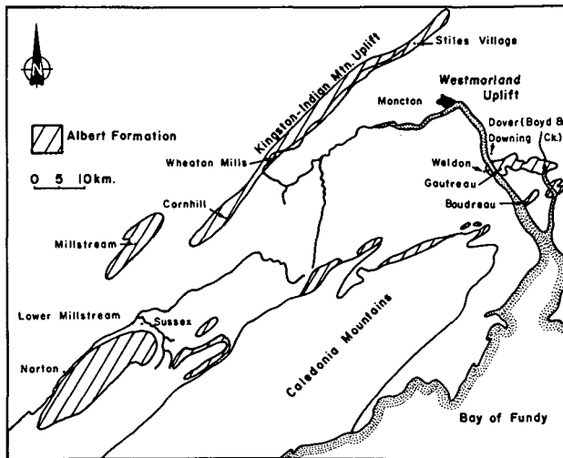
Fig. 2 - Surface outcrop of the Albert Formation in the Moncton Subbasin and location of bounding uplifts and localities referred to in the text (modified after Macauley and Ball 1982).
