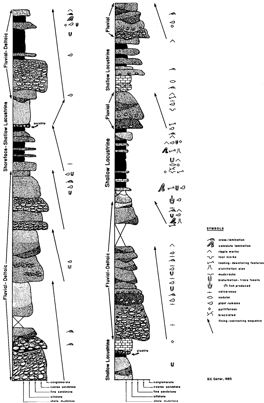
Fig. II - Stratigraphic section and environmental interpretation of the Albert Formation at Norton, Moncton Subbasin, southern New Brunswick. Vertical scale is 1cm = ca.5m (after Carter 1985).
