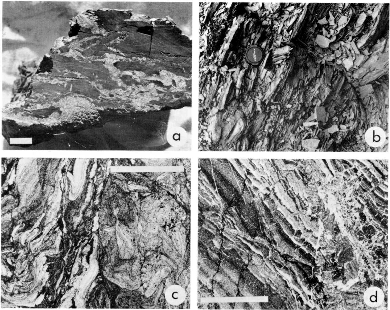
Fig. 7 - Marginal lacustrine lithofacies (carbonate mudflat), Albert Formation, Moncton Subbasin. a) Dark grey to black shale heavily veined by secondary orange brown calcite and ankerite. b) Thinly interbedded siltstone and shale, siltstones exhibiting small-scale cross-lamination and normal grading. Stratigraphic top to left. c) Highly contorted silty mudstone exhibiting syndeposition or pre-compaction deformation. d) Brecciated shale infilled by secondary calcite within both concordant and discordant veins and small-scale normal and reverse faults. All sections or samples from Indian Mountain. Bar scale in a, c and d is 1cm; lens hood in b is 50mm diameter. Photomicrographs c and d in transmitted light, parallel nicols.
