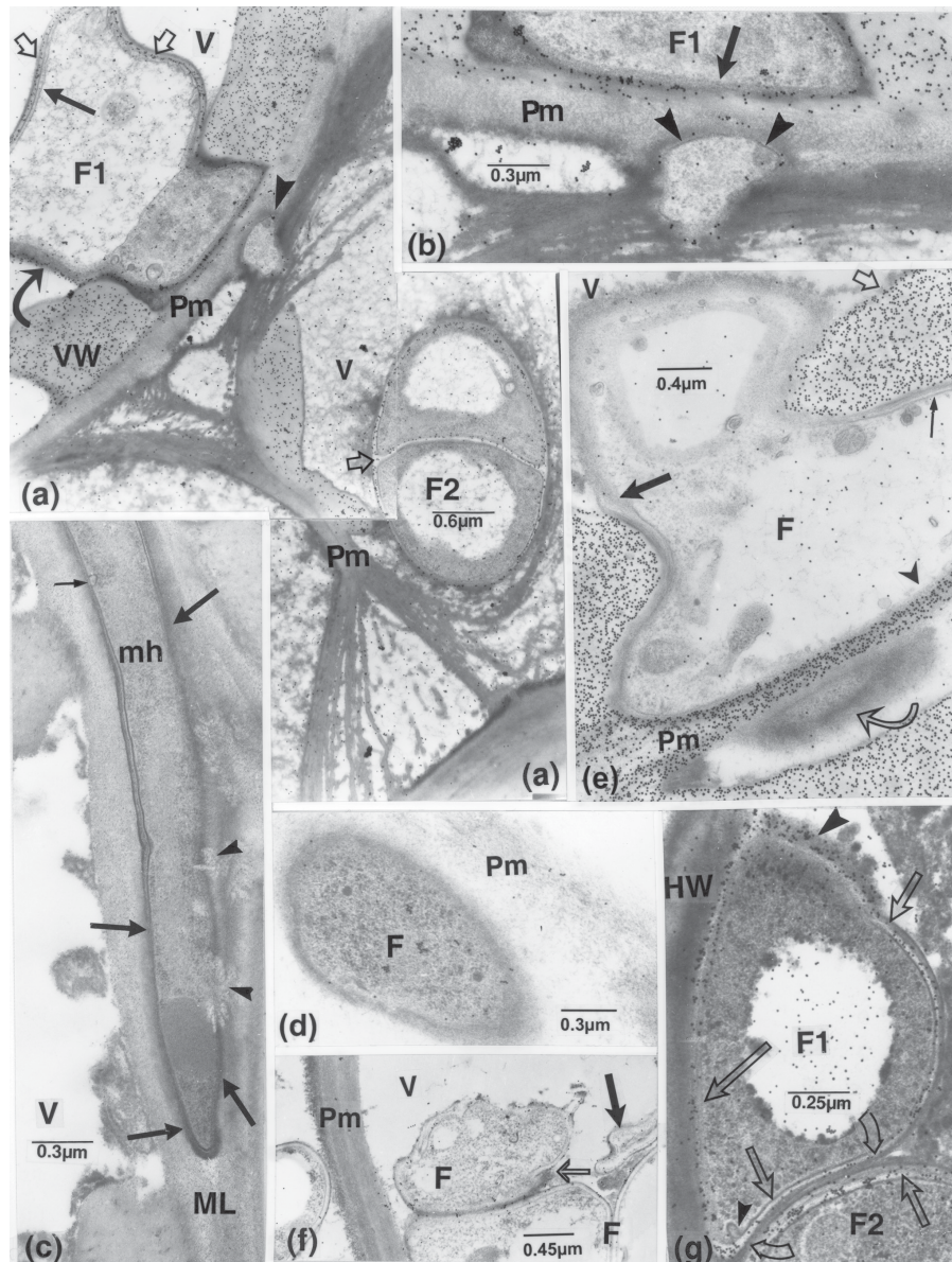
Figure 1. F, fungal cell; HW, host wall; mh, microhypha-like element; ML, middle lamella; Pm, pit membrane; V, vessel element; VW, vessel wall. (a and, enlarged portion, b): labelling for chitin is associated with: 1) the fungal lucent wall layers (light arrows), in cell F1, not to portions contacting the host walls. An inner double layer (straight, dark arrow) is present in the cell; 2) vessel secondary walls; 3) traces of fibrillo-granular matter in their lumina, and fungal cell vacuoles; and 4) the outer opaque layer (cell F1, curved arrow) (with its cytoplasm concentrated in the part filling the pit chamber) in portions close to or juxtaposed to the pit membrane. The inner fungal wall has a loosened appearance (arrow in b). The peg (arrowheads), in the pit chamber, is not delimited by a distinct wall, as indicated by its lack of labelling. The pit membranes are dislocated as shreds. (c): an aseptate intramural microhyphal element is seemingly locally delimited by only opaque bands (between thick arrows); these also appear to be discontinuous with signs of cell content invasion into the host wall (arrowheads). An incurving of the plasma membrane is discernible (thin arrow). (d): a lucent layer is not discernible in the intraparietal fungal cell (present in an altered pit membrane), demarcated by a layer of filamentous appearance. (e): labelling for cellulose. A fungal cell contouring a pit chamber shows a distinct, lucent layer in one portion (thin arrow); a thin and loosened layer along the labelled pit membrane (arrowhead); and a thicker layer seemingly becoming confluent with a more distended layer pervaded by opaque material (dark arrow); the latter is confluent with the coating (light, straight arrow). In the pit chamber of an adjoining vessel, an element (curved arrow), delimited by thin bands, and somewhat similar to that in d, is surrounded by a layer of fine filamentous matter. (f): a fungal cell wall is discontinuous or apparently overlaps at one point (light arrow). A collapsed hypha occurs nearby (thick arrow). (g): labelling for chitin is associated with fungal cell inner lucent layers (short, straight arrows). The region of cell F1 contacting the host wall has an imprecise lucent layer, with labelling mostly associated with outer opaque matter (long arrow) including a larger mass in a void space (large arrowhead) surrounding the cell; this irregular labelling is matched throughout by a non discernible plasma membrane, contrary to its clear presence elsewhere (between the short, light arrows). Bands of opaque matter and other fine components occur in the outer cell cytoplasm (in line with the large arrowhead), and a kink (small arrowhead) is visible in the plasma membrane. The outside opaque layers of cells F1 and F2 appear confluent at places (curved arrows).
