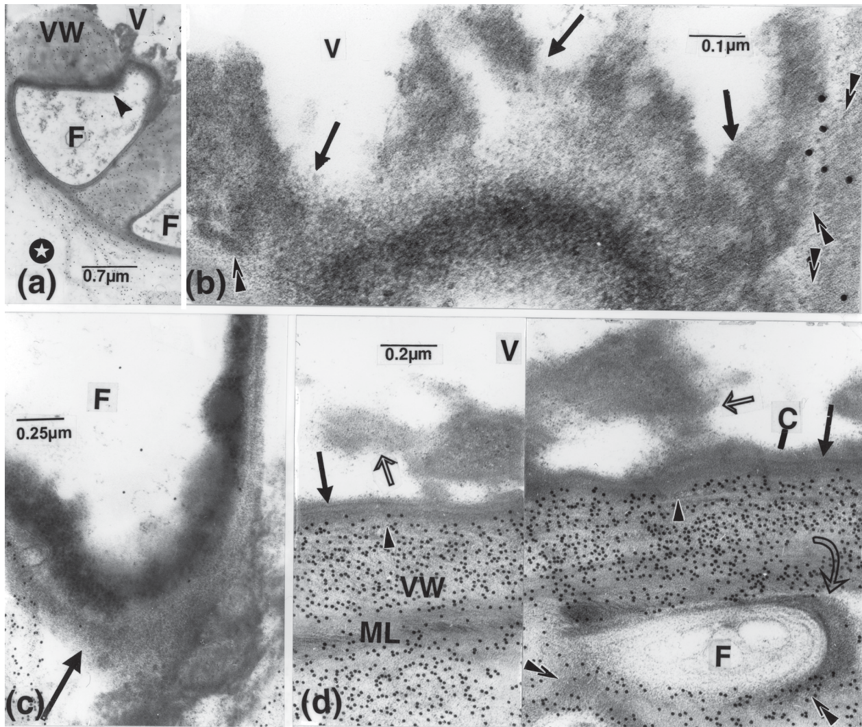
Figure 3. C, coating; F, fungal cell; ML, middle lamella; V, vessel element; VW, vessel wall. (a): labelling for cellulose. Fungal cells contour borders of opaque secondary thickenings. The pit membranes and adjacent host wall are altered (star). (b): enlarged portions from a (above the arrowhead). Filamentous structures stemming across the fungal wall and into the vessel lumen (arrows) extend into the vessel wall (superimposed arrowheads). (c): late stages of infection. Filamentous structures reach from the opaque matter present in an intracellular fungal cell to the matter surrounding it (arrow). (d): the compact coating, the mass of opaque matter connected to it (light arrows), and the extracellular material of the intraparietal fungal cell (curved arrow) contains fine filamentous structures extending into the host wall (superimposed arrowheads). The vessel wall displays similar structures (arrowheads) extending from the coating, containing paired bands (dark arrows).
