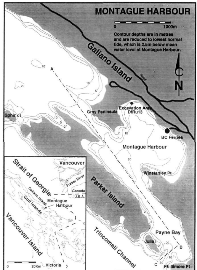
FIGURE 1. Map showing the location, physiography and bathymetry of Montague Harbour. Map was derived from Canadian Hydrographic chart no. 3473.
