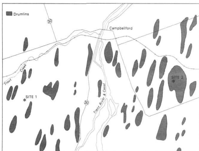
FIGURE 11. Location of site 2 related to site 1 at Trout Creek.
