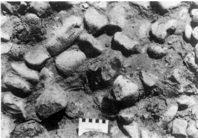
FIGURE 9. Matrix-rich cobble gravel; note graded bedding in the matrix above the scale (in cm).
