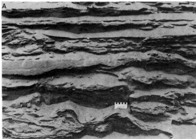
FIGURE 13. A) Lee-side sand and silt with pebbles (location d, Fig. 6). Silt layers are cohesive and stand out, whereas sand beds have been winnowed. B) Trough cross-bedded sand overlain by tabular cross-bedding in gravel (location f, Fig. 6). C) Graded and cross-bedded sand with syndepositional slump failure (location g, Fig. 6). Arrow marks failure plane. Plane beds (P).
