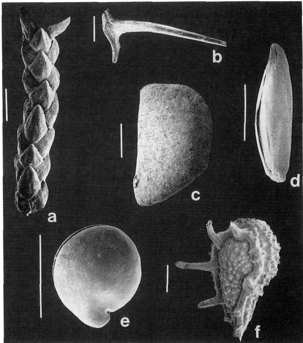
FIGURE 5. Scanning electron micrographs of selected plant macrofossils recovered from the middens. a) Juniperus scopulorum branch; b) Rosa thorn; c) Arctostaphylos uva-ursi seed; d) Poaceae seed; e) Chenopodiaceae seed; f) Lappula redowskii -type seed. Scale bar represents 1 \mu\text{m} .
