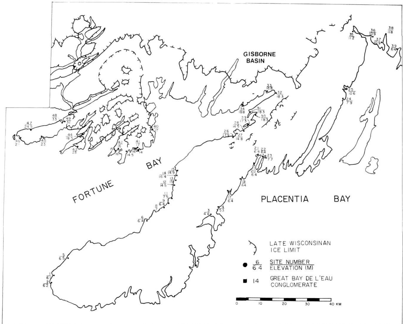
FIGURE 3. Late Wisconsin ice marginal position and elevations of the Late Wisconsin marine limit in the Burin-Hermitage area of southern Newfoundland. The datum is higher, high water level of large tides.
