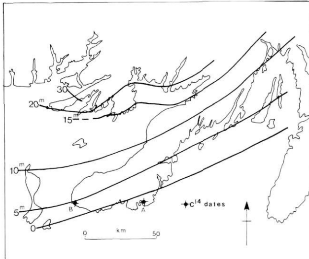
FIGURE 4. Isopleths of postglacial emergence in the Burin-Hermitage area of southern Newfoundland and the islands of St. Pierre and Miquelon.
