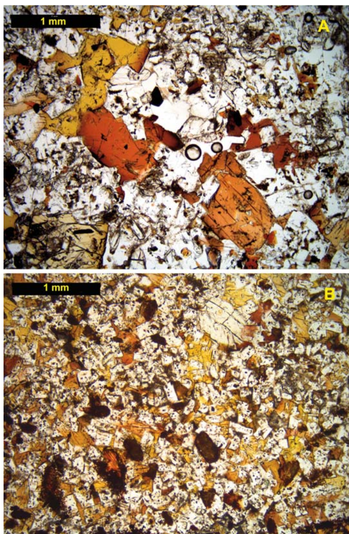
Figure 3. Examples of sanidine amphibole lamproite showing the characteristic lemon-orange to orange-brown pleochroism of groundmass poikilitic K-Ti-richterite. (A) Cancarix Sill (Murcia-Almeria Province) with colourless co-crystallizing potassium feldspar. (B) Moon Canyon (Utah) with microphenocrystal sanidine set in a matrix of K-Ti-richterite.
