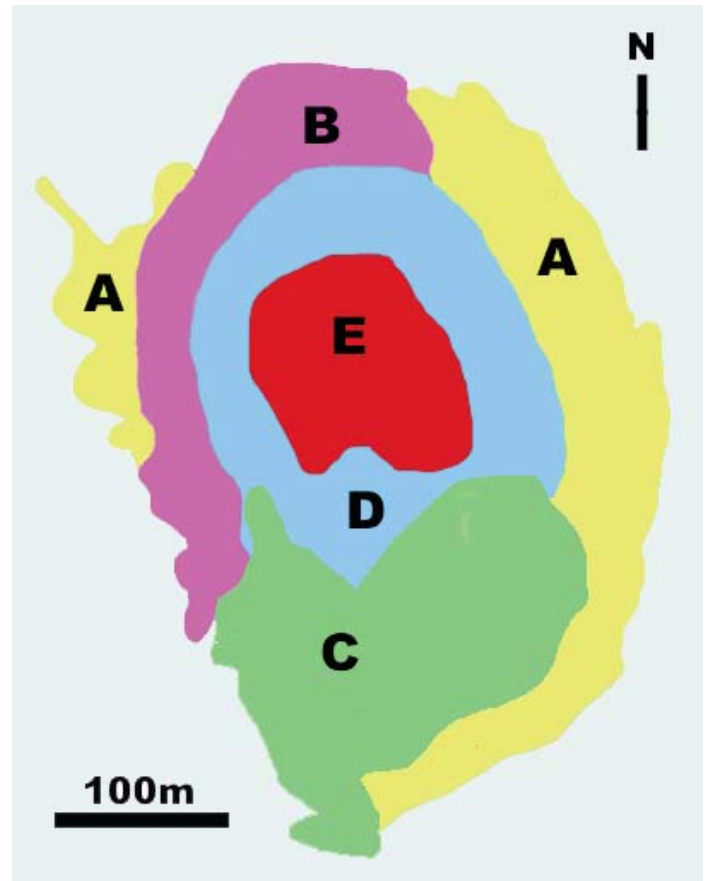
Figure 17. Outcrop plan of the Majhgawan lamproite illustrating the disposition of the pyroclastic units (after Mathur and Singh 1971; Rao 2007). A = yellow-green heterolithic pyroclastic breccia; B = yellow-brown heterolithic pyroclastic breccia; C = heterolithic breccia; D = mica-rich pyroclastic breccia; E = mica-free breccia. Note that these units require re-investigation and reclassification (see Fig. 18).
