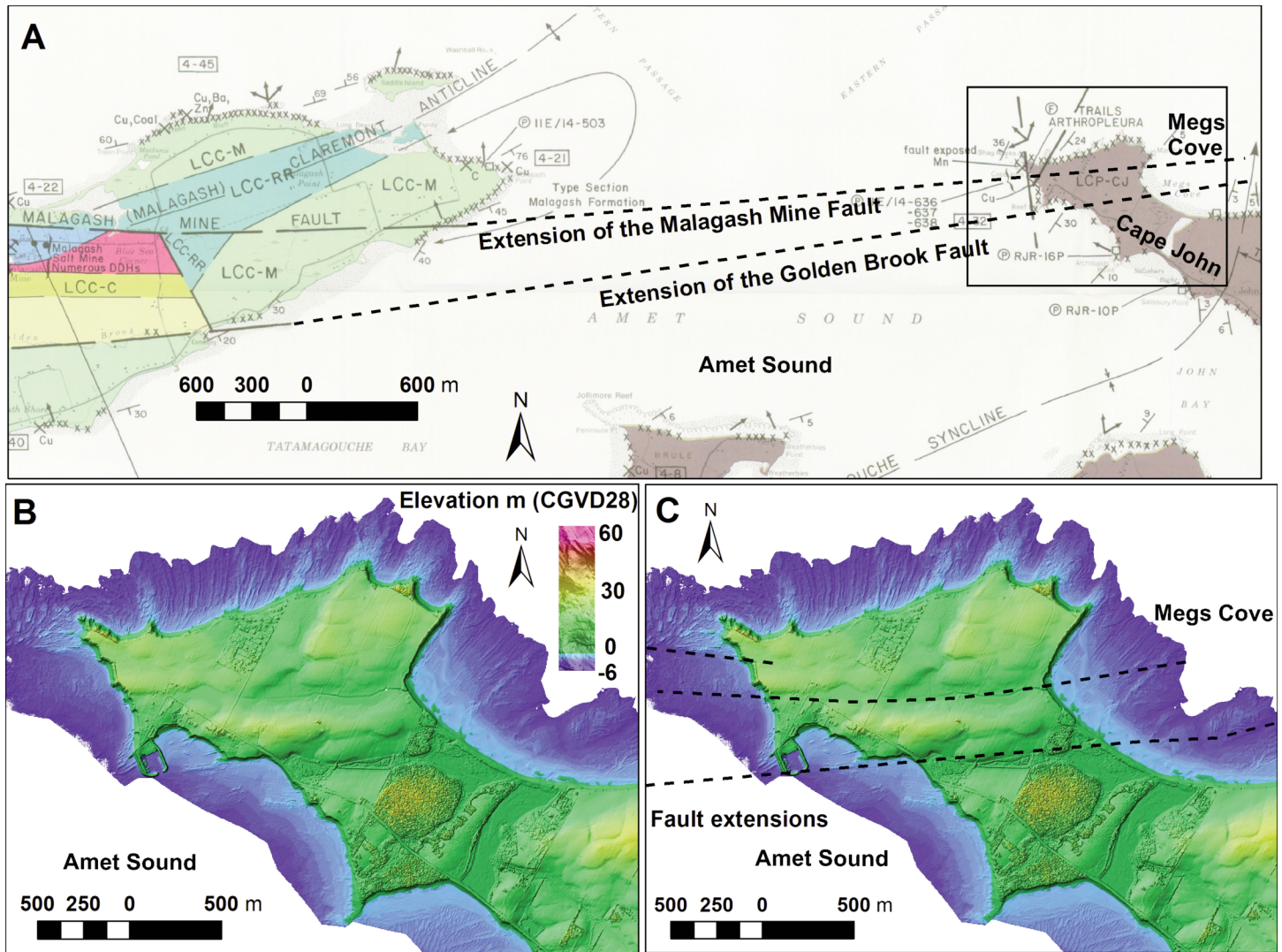
Figure 9. A. Projection of the Malagash Mine and Golden Brook faults to Cape John, with lidar map location outlined in black. Geology is from Ryan and Bochner (1994). B. Lidar Digital Surface Model (DSM) of the area enclosed by the black rectangle in A. C. Lidar DSM with interpreted fault extensions (black dashed lines) following the onshore lineaments.
