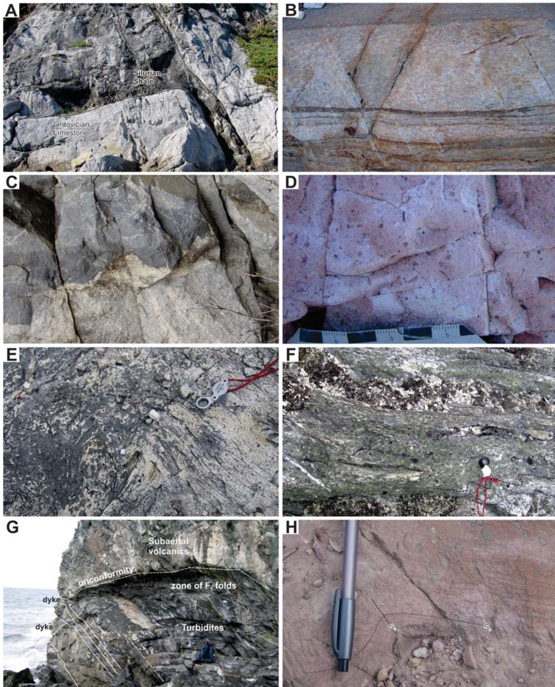
Figure 4. Representative photographs of Silurian rocks along and east of the Red Indian Line. A. Darrivilian limestone blocks in a matrix of Silurian shale of the Joey's Cove mélange at Rogers Cove, New World Island (see Reusch 1987). B. Contact metamorphosed Badger Group turbidites adjacent to the Dawes Pond Granodiorite and Hodges Hill Batholith. Note bedding subparallel to foliation. Nearby outcrops of the Roberts Arm Group preserved evidence for polyphase deformation. C. Twin Lakes phase of the Hodges Hill Batholith displaying scalloped contact between mafic and felsic phases, suggesting they are co-magmatic. D. Pristine hypabyssal quartz-phyric rhyolite of the Dawes Pond Granodiorite. E. Foliated Stony Lake rhyolite deformed into symmetrical folds in hinge of anticline. Folds are accompanied by weak axial planar cleavage. Hand lens for scale. F. Strongly foliated ca. 423 Ma Stony Lake rhyolite. Foliation is tectonic and folded by younger mesoscopic folds containing a weak axial planar cleavage (lower right corner). Hand lens for scale. G. Unconformity between Salinic ( F_1 ) deformed Badger Group turbidites and subaerial volcanic rocks of the Port Albert Formation of the Botwood Group. Turbidites below the unconformity contain a zone of F_1 folds (Karlstrom et al. 1982) and are overlain by a thin conglomerate layer that locally contains pebbles with pre-entrainment cleavage. Both units are folded by NW-verging Acadian(?) structures ( F_3 of Lafrance and Williams 1992). H. Folded and cleaved red beds of Wigwam Formation near the contact with the overlying Stony Lake Formation felsic volcanic rocks.
