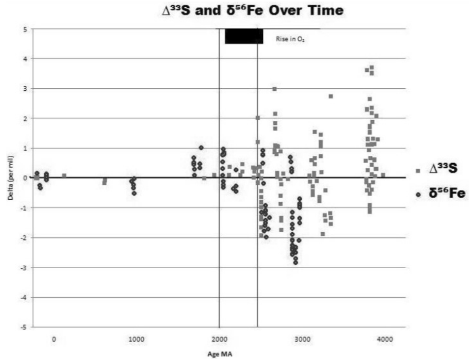
Figure 3. Ranges of \Delta^{33}\text{S} (%) (Farquhar and Wing 2003) and \delta^{56}\text{Fe} (%) (Rouxel et al. 2005) over time. The rise of atmospheric oxygen is demonstrated by dramatic decreases in the ranges observed in both isotopic systems.
