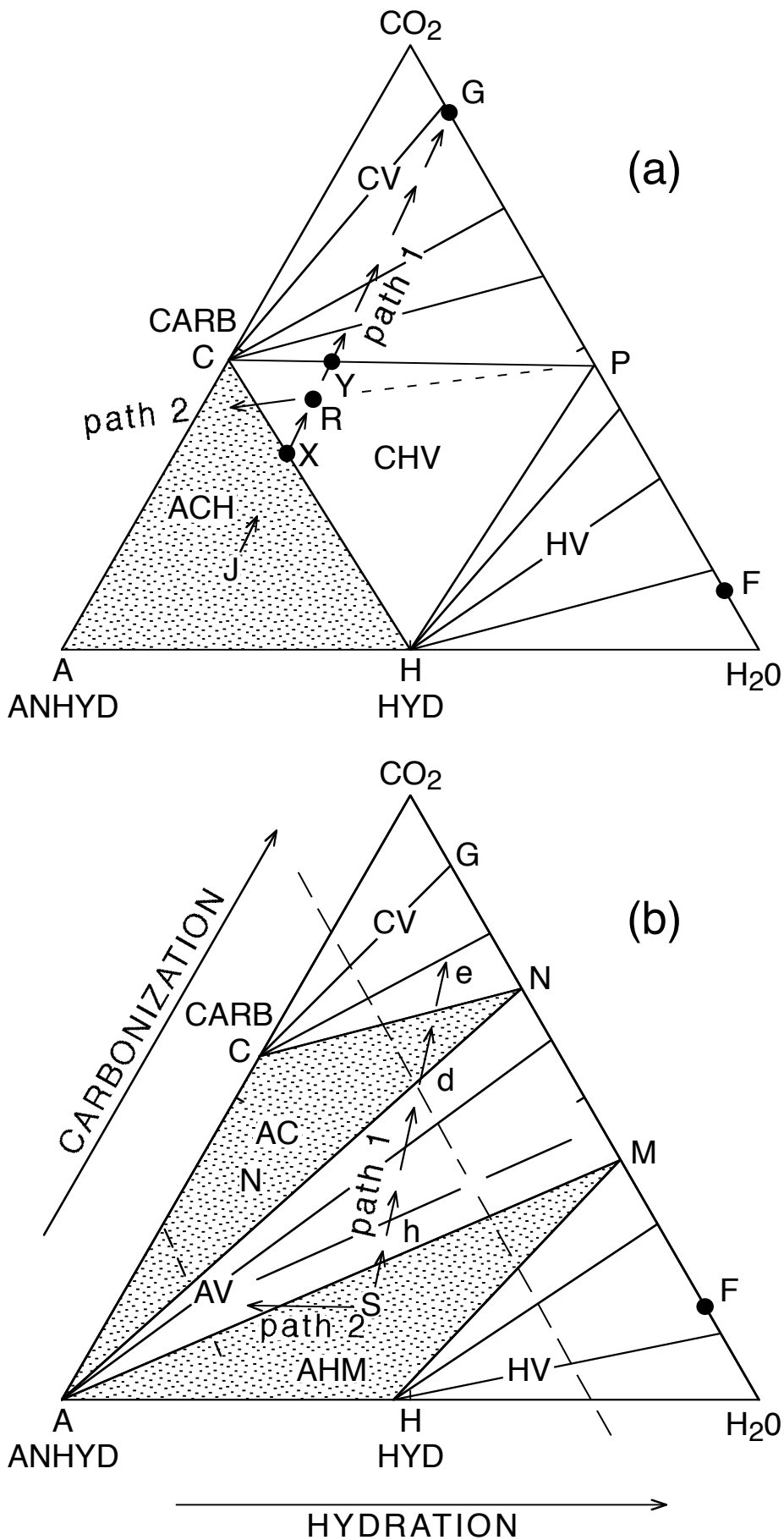
Figure 9. The effect of the introduction of fluids into a potential source rock (see Murphy 1989). Schematic representation depicting phase relationships between a volatile-absent phase A, a hydrous phase H, a carbonate phase C and fluid. Modified after Egglar (1978). The stippled triangle in (a) represents the fluid-absent region (see Thompson 1983) and the stippled triangles in (b) are zones of invariant vapour composition (Egglar 1978). Within the stippled triangles of (b) fluid composition is held constant during influx of exotic fluid by re-adjustment in the modal abundances of the phases at the apices of the compositional triangle.
