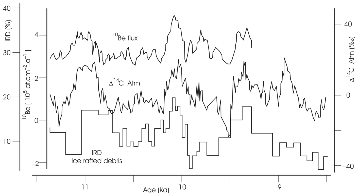
Figure 10. The borehole record (Bond et al., 2001) of ice rafted debris (IRD), which is a climate proxy, and the coeval record for CRF proxies, 10 Be in sediments and Δ 14 C in growth rings of trees. Adapted from Kromer et al. (2001).
