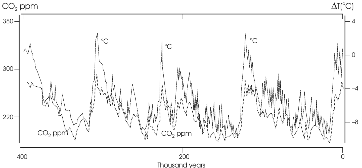
Figure 7. Antarctic (Vostok) ice core data for the last 400,000 years. Temperatures (dashed curve) are derived from oxygen and hydrogen isotopes of ice and \text{CO}_2 concentrations (dotted curve) were measured in frozen air bubbles. Adapted from Petit et al. (1999).
