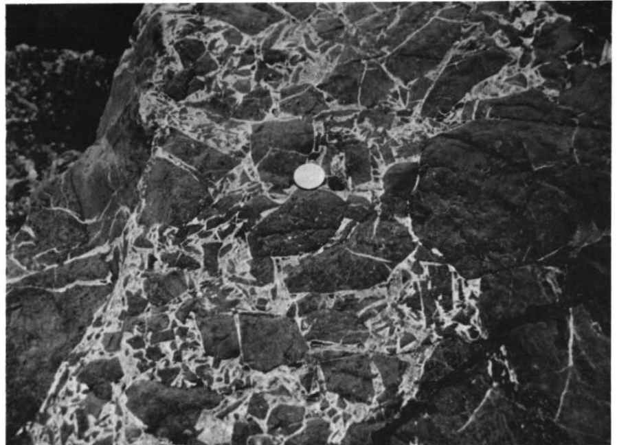
Figure 14 A collapse breccia of subtidal lime mudstone clasts in white calcite; caused by the solution of anhydrite at the top of a shallowing-upward sequence in the Shunda Fm. (Mississippian) at Cadomin, Alberta (photo courtesy R. W. Macqueen).
