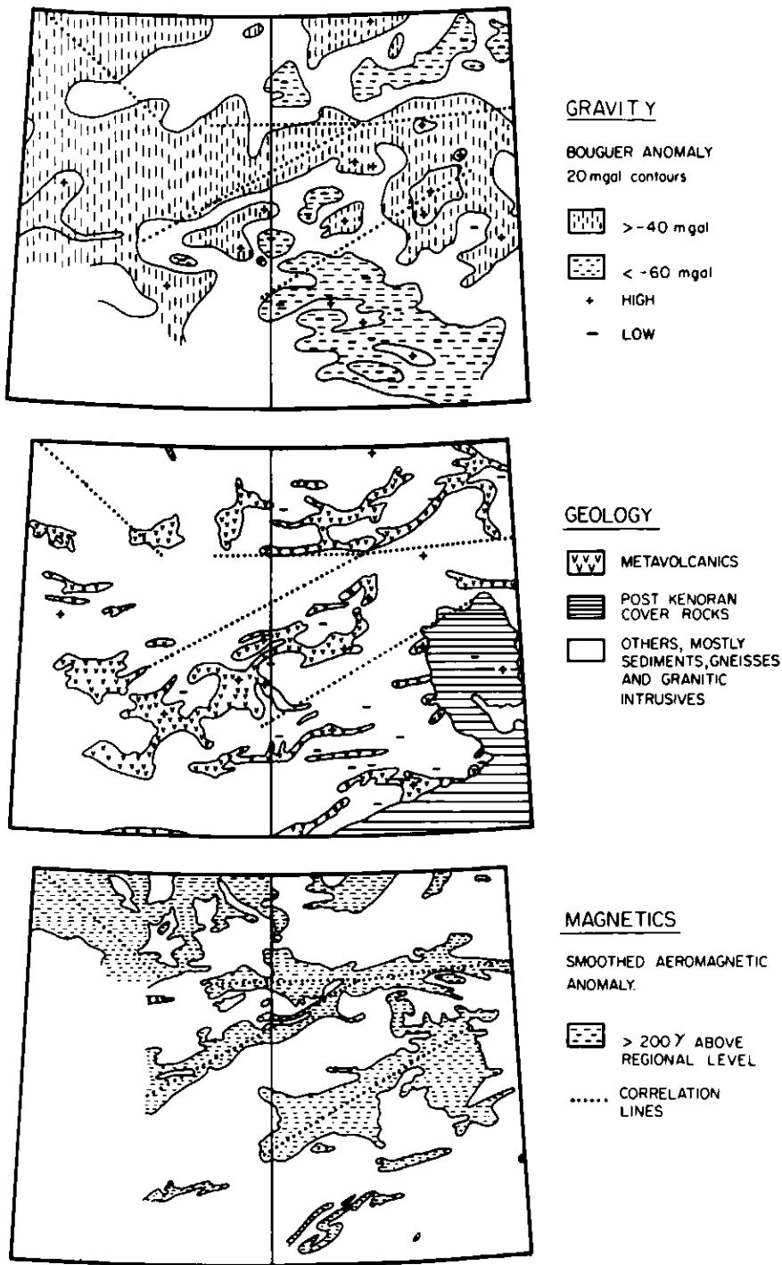
Figure 6 Regional geology, gravity and magnetics in the vicinity of the Geotraverse corridor. To aid in the correlation of the three maps, a series of dotted reference lines have
