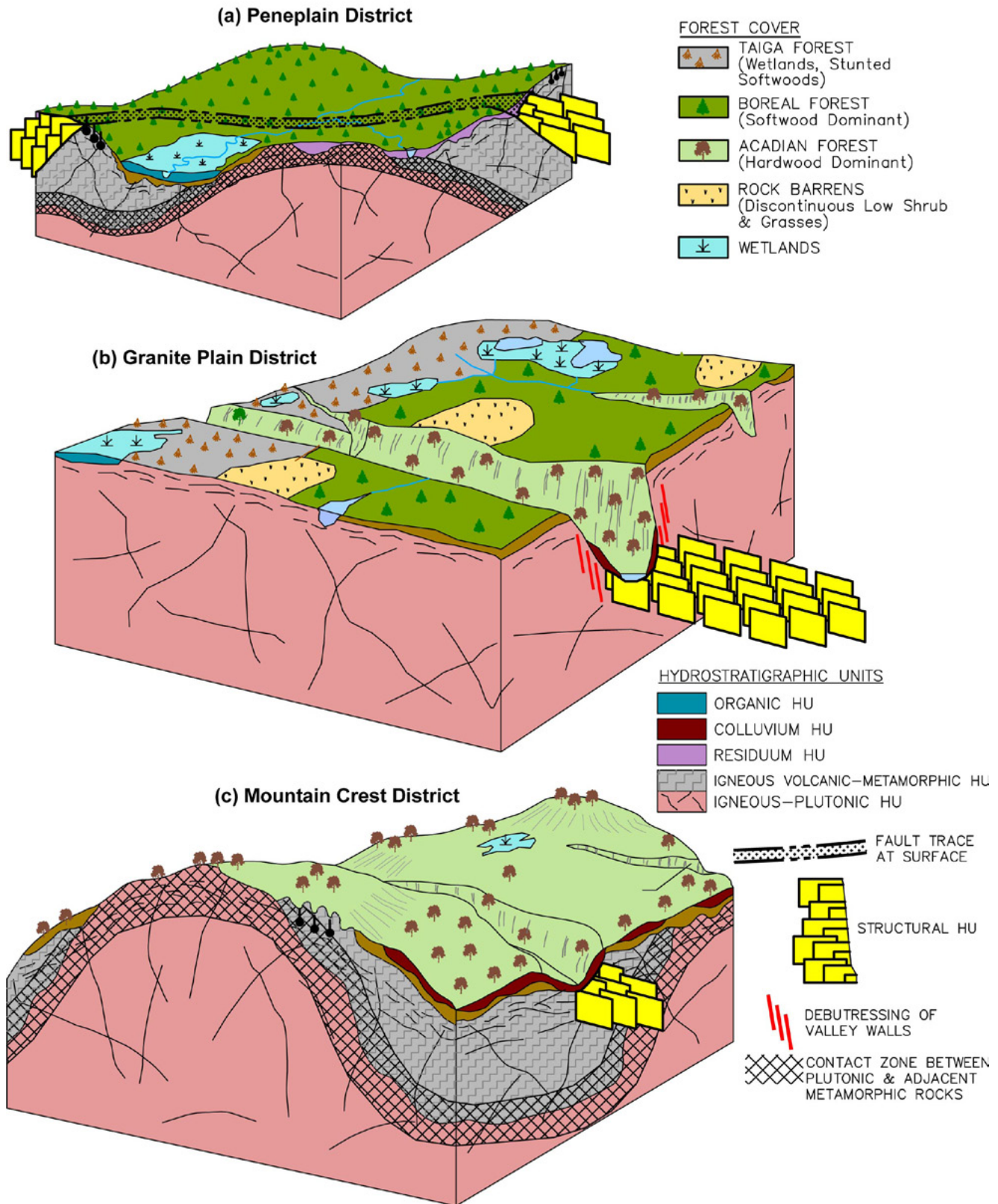
Figure 5. Conceptual 3-D block models for faults and other features in the Highland Hydrological Region in (a) Peneplain District, (b) Granite Plain District, and (c) Mountain Crest District.
