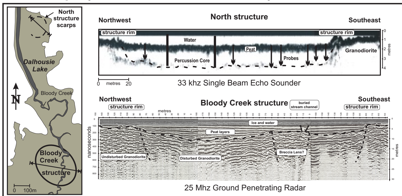
Figure 2. Survey and interpretation of the morphometry of the North structure depression and, for comparison, the Bloody Creek structure depression. Sub-bottom sonar traverses were obtained when the sites were flooded. 33 khz sonar, probing and percussion coring confirm the crater morphometry of the North structure and its similarity to the Bloody Creek structure. Both structures are infilled with post-glacial peat and lacustrine sediments.
