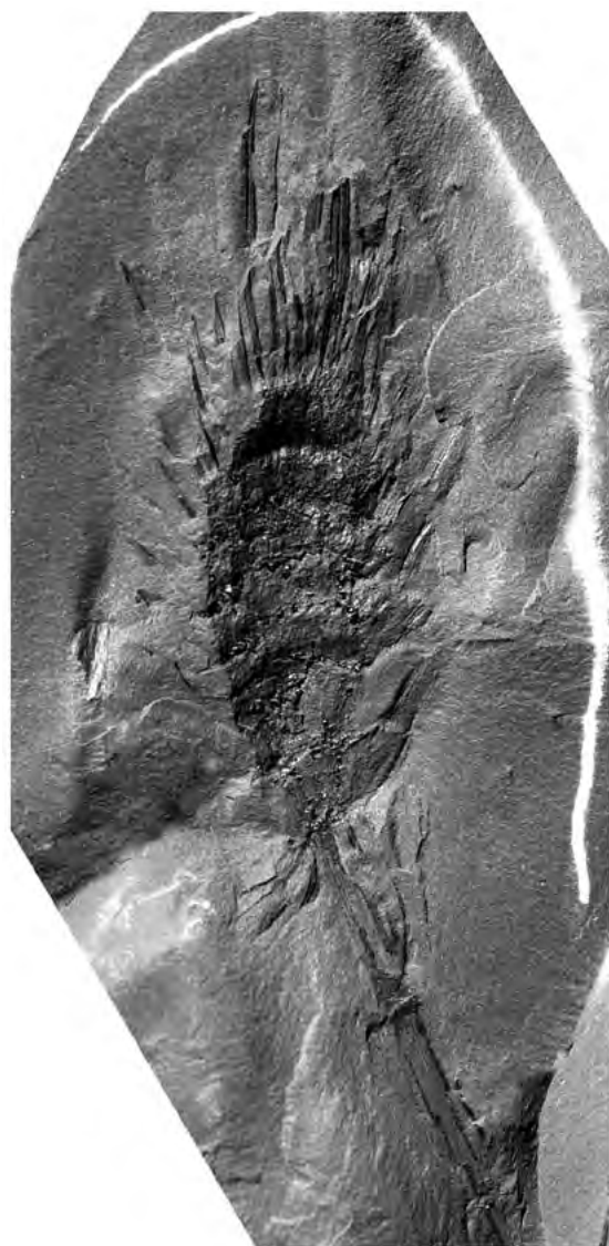
Figure 17. Acrobullbillites sp. (× 2). GSC 9017. Specimen figured by Bell (1944, pl. LXXI, fig. 1) as Asterophyllites equisetiformis . Origin: Springhill, No. 2 mine, from roof shales in waste dump (locality 1039), Nova Scotia. Repository: Geological Survey of Canada, Ottawa.
