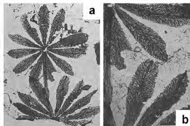
Figure 6. (a) Annularia latifolia (× 3). Reproduction of the type of Annularia jongmansii as figured by Walton (1936, pl. 31, fig. 12) (so as to show the identity with Dawson's species). Origin: Devon Tower Colliery, southwest of Tilli-coultry, Clackmannanshire, Scotland. (b) Annularia latifolia . Detail of specimen in Fig. 6a as figured by Walton (1936, pl. 31, fig. 13) showing the reticulate cell pattern of the lamina.
