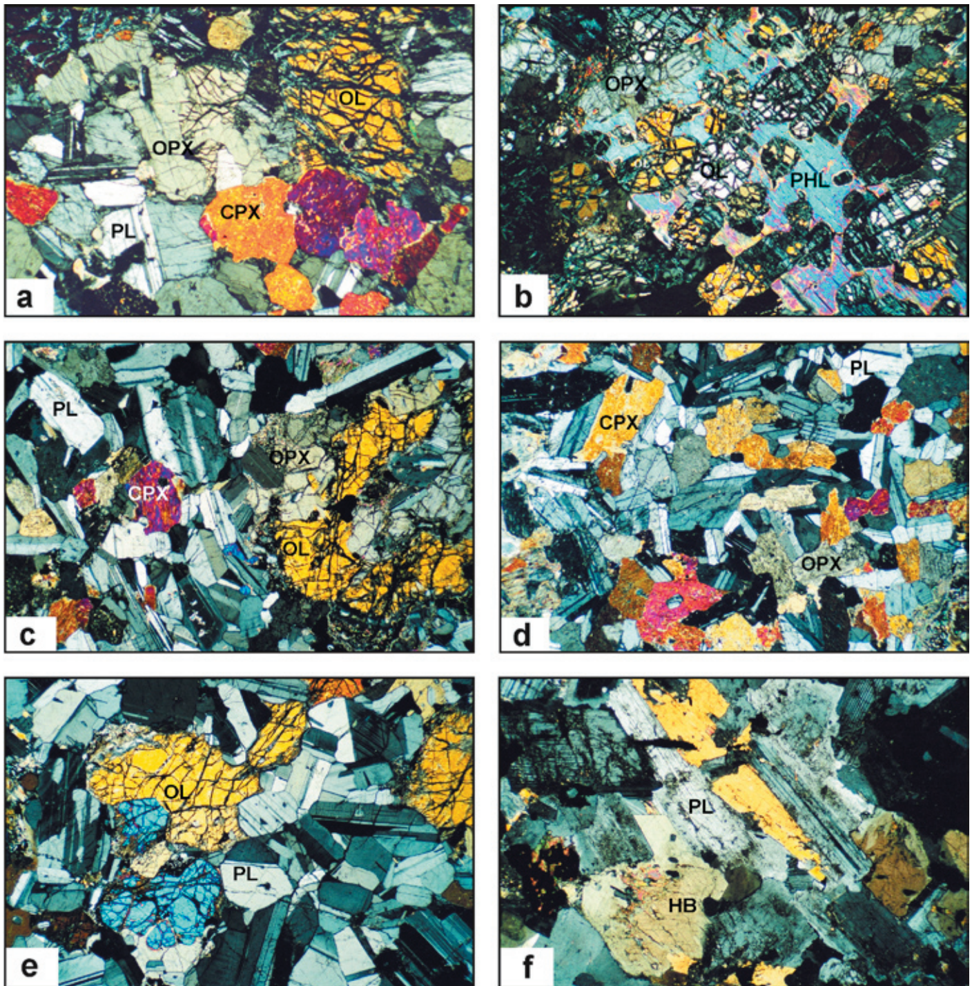
Fig. 4. Photomicrographs showing examples of lithologies in the MSP. (a) Plagioclase-bearing lherzolite (sample RH03-64). (b) Olivine websterite with phlogopite (sample RH03-84). (c) olivine gabbro-norite (sample RH03-57). (d) Medium-grained gabbro-norite (sample RH03-57). (e) Troctolite (sample RH03-100). (f) Diorite (sample MS-230). All photographs are under crossed polars. Width of field of view is 4 mm. Symbols: CPX, clinopyroxene; HB, hornblende; PL, plagioclase; OL, olivine; OPX, orthopyroxene; PHL, phlogopite.
