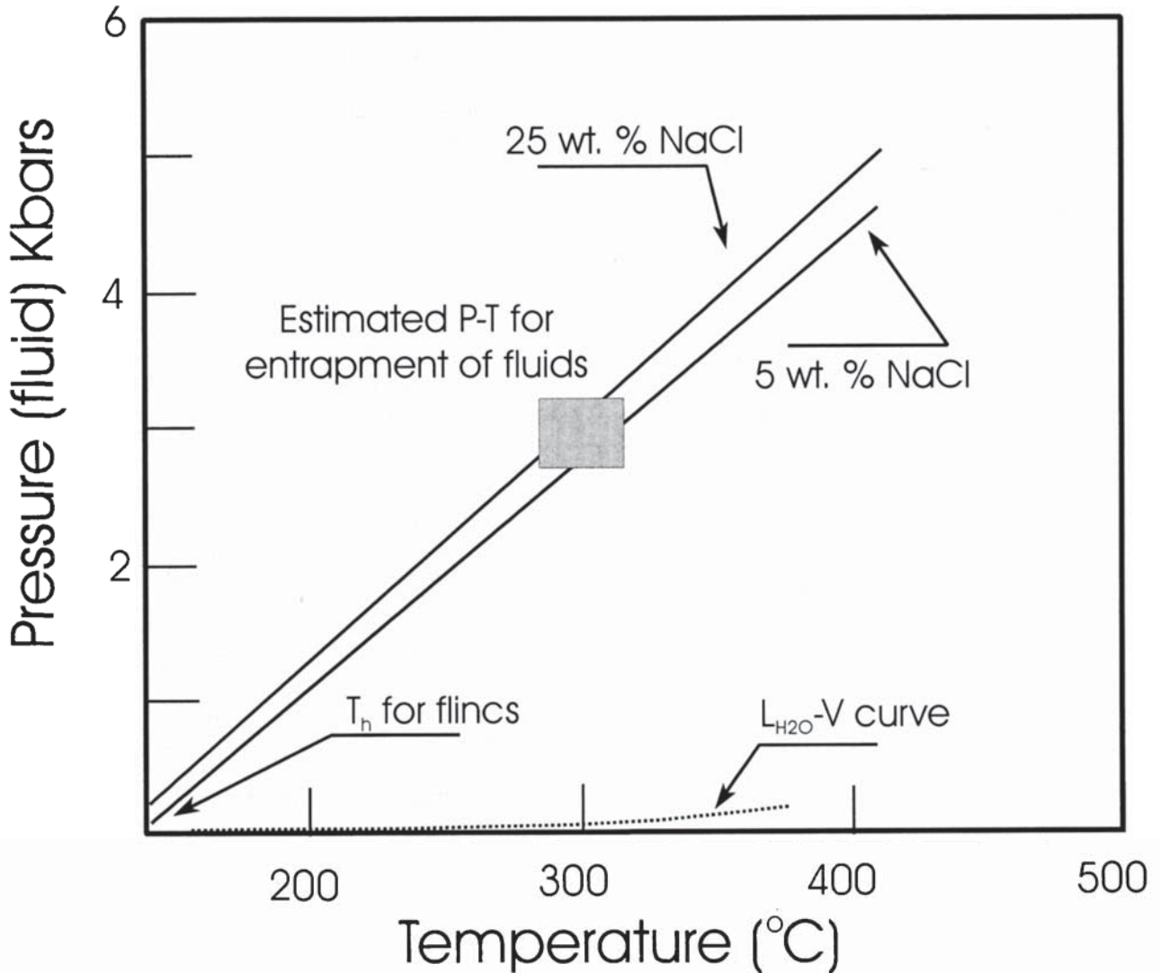
Fig. 16. Pressure-temperature plot showing the projection of isochores for fluid inclusions from Dunbrack and the estimated conditions of entrapment for the fluids based on discussions in the text. The two lines are for 5 and 25 wt. % eq. NaCl aqueous inclusions that homogenized at 140°C; isochores constructed using the program FLINCOR (Brown 1989). The isochores represent the NaCl-H 2 O type fluids which form the most abundant fluid inclusion population at Dunbrack.
