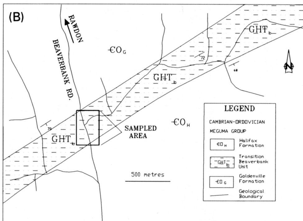
Fig. 1. (A) Generalized geological map of central Nova Scotia showing the location of North Beaverbank; (B) Detailed geological map of the study area, Beaverbank Road section, North Beaverbank.
