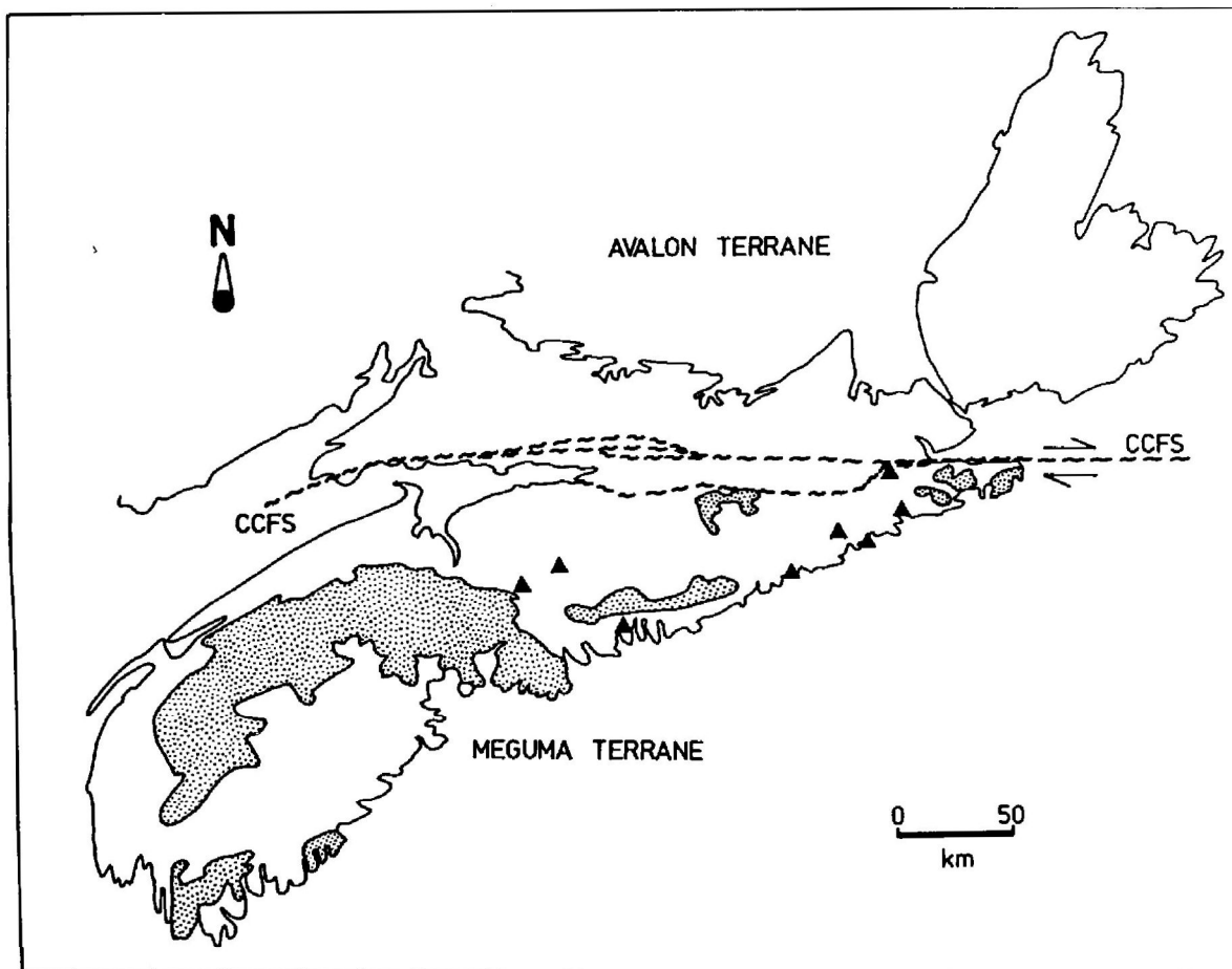
Fig. 1 - Meguma Terrane of Nova Scotia, solid triangles show localities of studied quartz veins. CCFS - Cobequid-Chedabucto Fault System. Stippling indicates major granitoid bodies.
