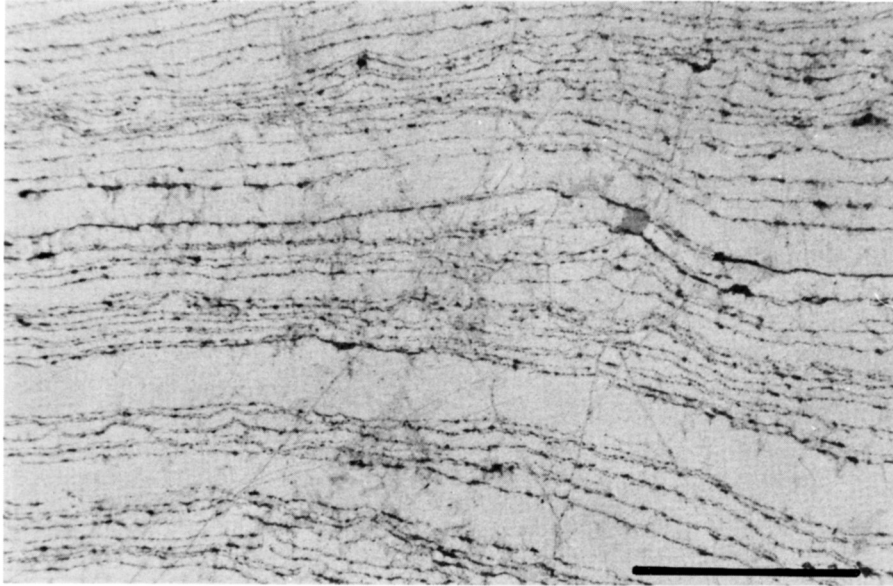
Fig. 7 - Phyllosilicate lamination. Sample from Renfrew. Scale bar = 1 mm.
