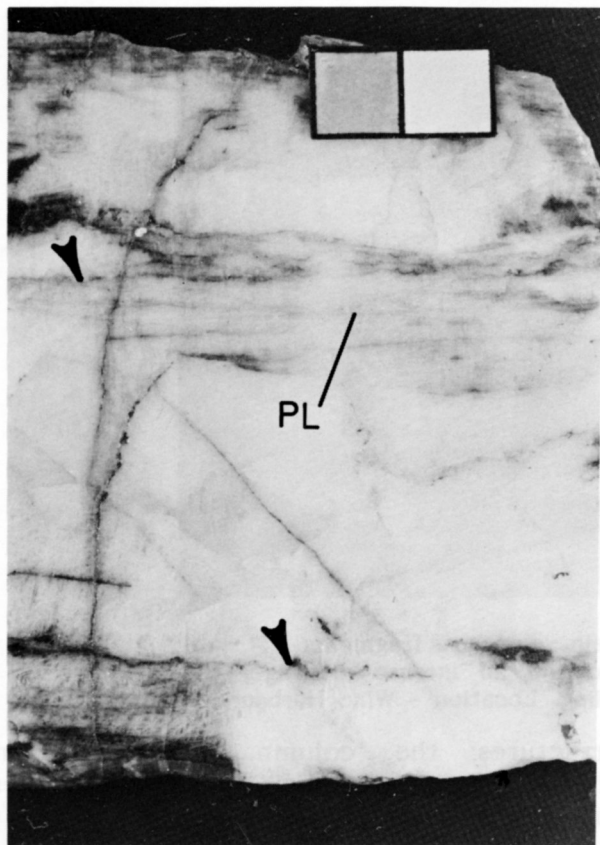
Fig. 3 - Sawn face of sample, phyllosilicate laminae indicated (PL). Note jagged structures (arrowed) which truncate phyllosilicate laminae. Sample from Harrigan Cove. Scale = 2 cm.
