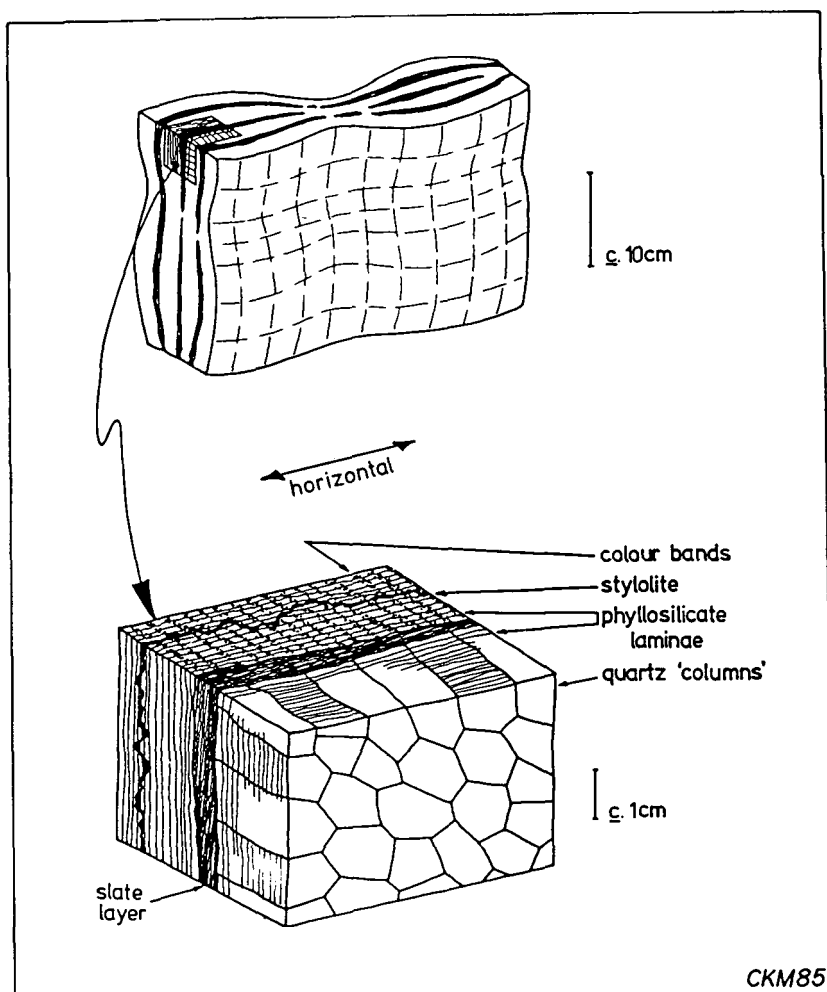
Fig. 5 - Idealized synoptic diagram of structural features of the bedding-concordant quartz veins.
