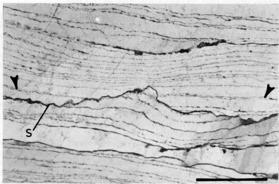
Fig. 8 - Jagged planar structure (stylolite, marked S). Note that this structure truncates the phyllosilicate lamination (one truncated lamina is arrowed). Sample from Renfrew. Scale bar = 1 mm.
