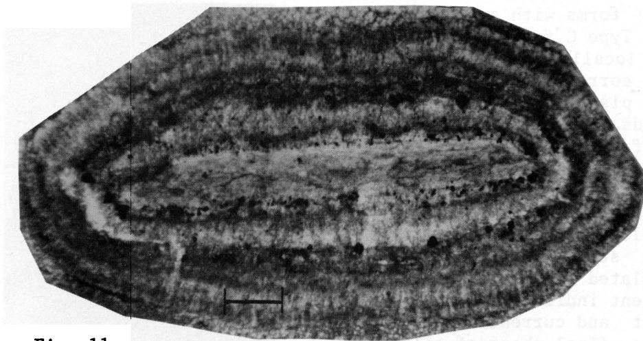
Fig. 11 Type C form encrusting an ostracode fragment. Scale bar 0.1 mm. Photomicrograph.
