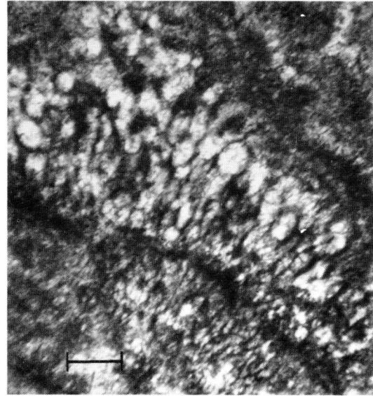
Fig. 6 Algal filaments (of unknown affinities). Scale bar is 0.1 mm. (Photomicrographs).
