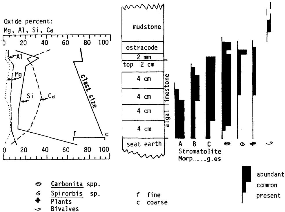
Fig. 7 - Variation of oxides (wt. percent) Mg, Ca, Si and Al, stromatolite growth forms and various clast types in relation to stratigraphy.
