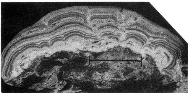
Fig. 9 Detail of alternating lamination of Type B morphology. Photonegative of a thin section. Scale bar 10 mm.
