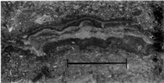
Fig. 8 Type B morphology attached to a calcareous substrate. Polished surface. Scale bar 10 mm.
