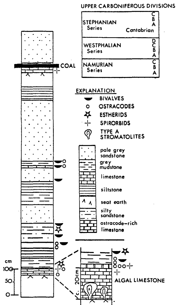
Fig. 2 - Generalized succession of strata at Lingan and Upper Carboniferous series.
