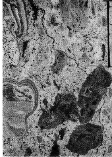
Fig. 10 Photonegative of algal limestone containing large irregular siltstone and micrite clasts, occasionally encrusted with Type B morphologies. Matrix contains abundant Type C morphologies in grain to grain contact. Scale bar 10 mm.
