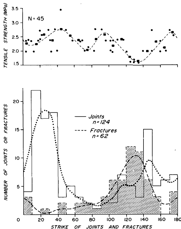
Fig. 3 - Joints, preferred fracture orientation and tensile strength in the flat-lying Pictou Formation near Cavendish, Prince Edward Island. Solid circles are individual tensile strength measurements, solid squares are averages per ten degree azimuth interval. In the histogram, the smoothed distribution curve for joint strikes is a dotted line, and that for preferred fracture azimuths is a broken line. Preferred fracture orientation correlates approximately with the strike of the 145° (nonsystematic) joints. The tensile strength minimum at 075° has no joint equivalent.
