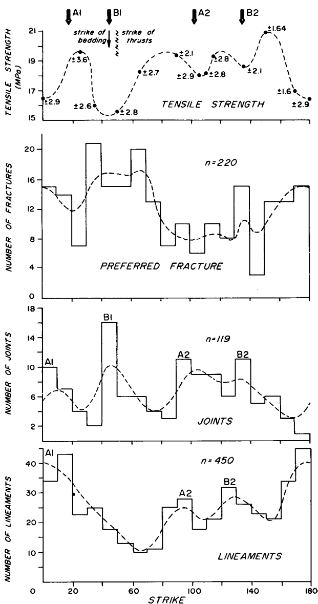
Fig. 8 - A comparison of trends displayed by tensile strength, preferred fracture, joints and airphoto lineaments in the McCoy Head Formation east of Gardner Creek, New Brunswick. Solid circles are means of 15 individual measurements. Standard deviations are shown for each mean. The solid arrows are the strikes of the joints in the two orthogonal joint systems in the outcrop shown in Figure 7 (lower photograph). There is a tensile strength minimum parallel to each joint set, but the strongest minima correlate with the joint sets A1, B1. There is no lineament trend parallel to the B1 joints. Broken lines are smoothed distribution curves.
