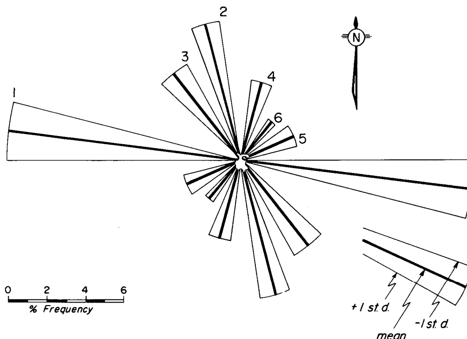
Fig. 10 - Airphoto lineament trends in the region east of Saint John, New Brunswick (after Naing 1976). The compilation includes all rocks.
