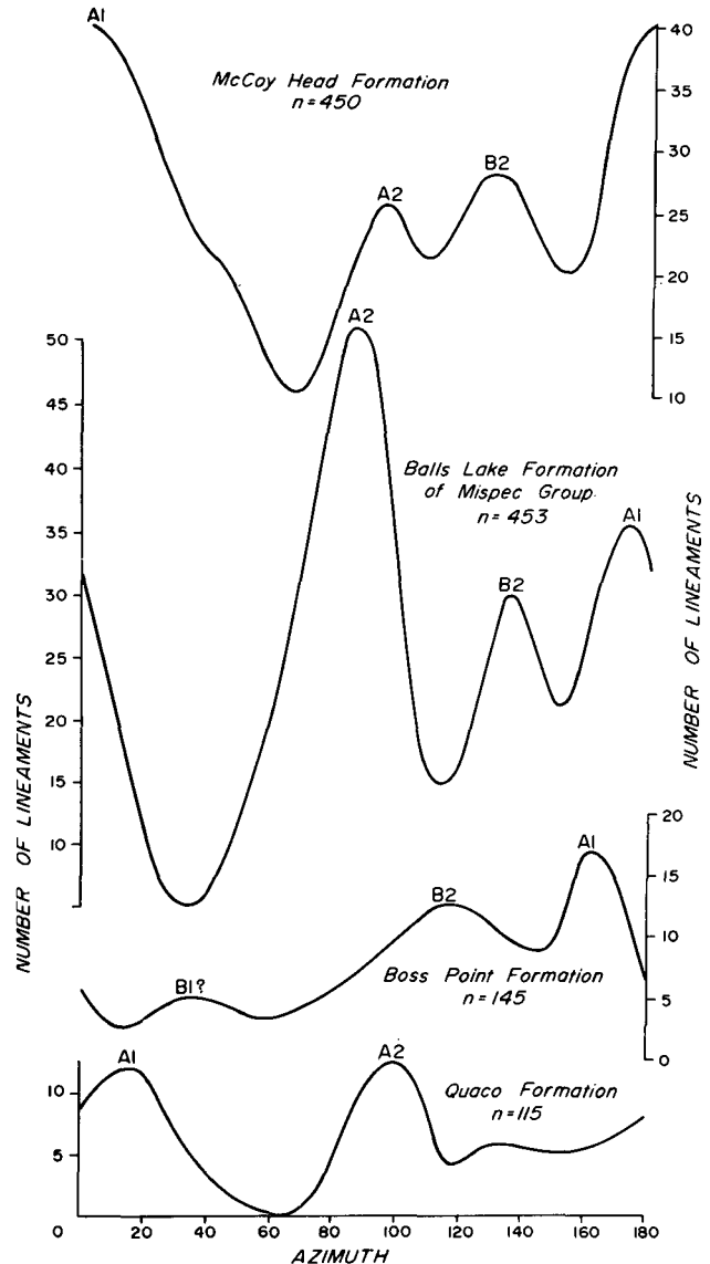
Fig. 9 - Airphoto lineament trends in four formations. The top three formations were affected by the Variscan-Appalachian orogeny. The A1, A2 and B2 lineament trends correlate approximately with the strike of corresponding joints in the Balls Lake and McCoy Head Formations (Figs. 2 and 8), but a lineament parallel to the B1 joints is missing. The Triassic Quaco Formation shows lineaments parallel only to the A orthogonal joint system. (After Naing and Lajtai 1977).
