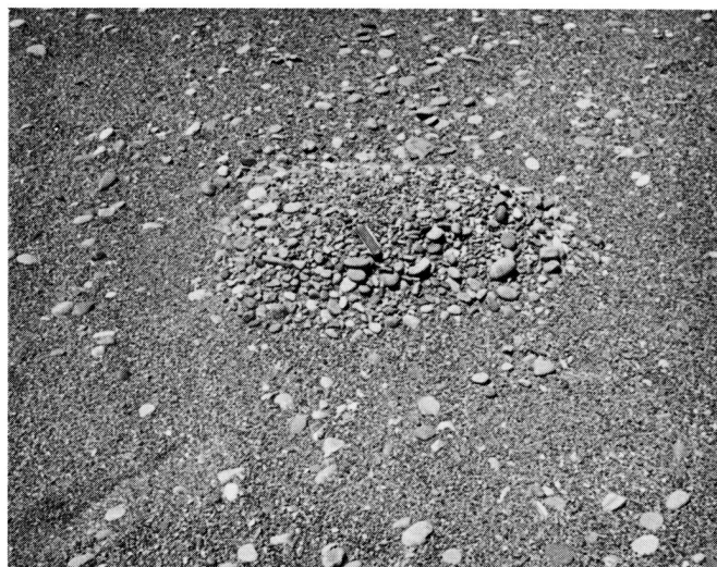
Fig. 3. A mature gravel cone exhibiting flat top and graded sides.
