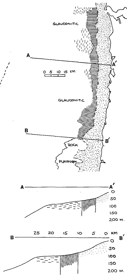
Fig. 1 (a) Diagram showing geomorphic zonation of a beach to inner shelf profile. (b) Plan and sectional views of two modern inner shelf areas, the low-energy Atlantic coast and the high-energy, wave-dominated Oregon coast.
