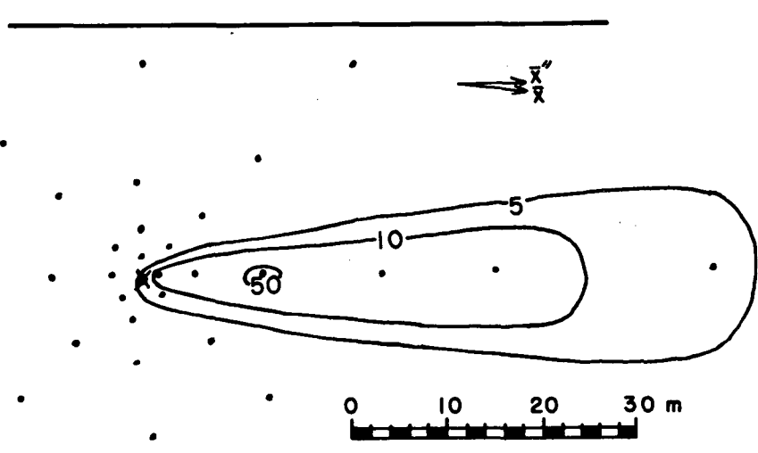
Fig. 14. Dispersal station D5: All notation as on Figure 11. Top: 1 day after injection; Bottom: 8 days after injection.
