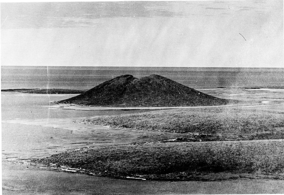
Figure 1: Pingo rising out of the flat landscape near the village of Tuktoyaktuk, Northwest Territories. (Photograph by Roger Belanger, Atlantic Oceanographic Laboratory, Dartmouth, Nova Scotia, Canada).
