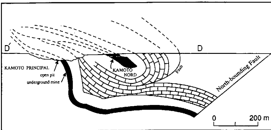
Figure 8 (a) (upper) Plan view of a portion of the Kolwezi mining district, showing the deformed and tilted megabreccia blocks hosting the Kamoto Principal, Kamoto Nord and Kamoto Etang mines. Economic mineralization is hosted by the basal portions of the Kamoto Dolostone (dotted patterns) and S.D. Formation (white). Section D-D' is illustrated in Figure 8b. From Demesmaeker (1963). (b) (lower) Profiles through the stratigraphy of the Kamoto Principal and Kamoto Nord mines (for location, see line D-D' of Figure 8a).
